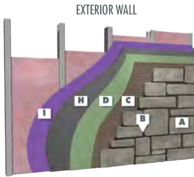
EXTERIOR WALL Framed wall with exterior rated sheathing – cement backer board substrate
