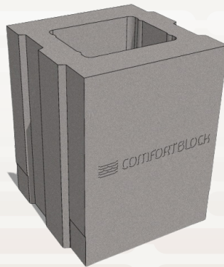
CB-6 Half 6"w X 8"H x 6"L
